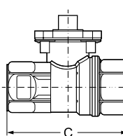
Two-way Valve
